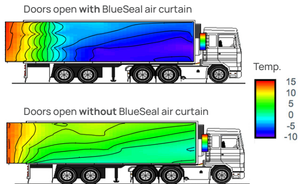
Heatmap tests after 10 minute door opening. Performed at a Dutch food logistics company
